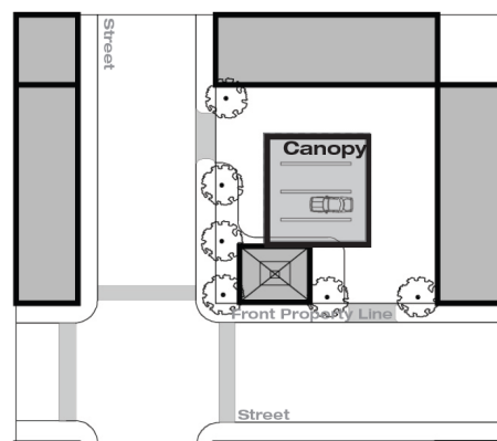
Figure 50-22.6-A: Relationship between the principal structure and the pump islands
